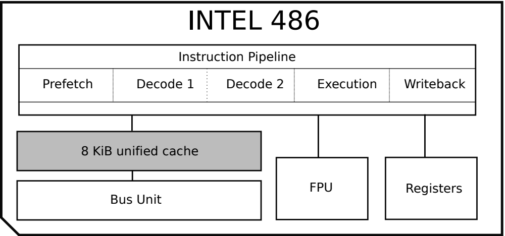
Figure 2.5: Intel 486 architecture
